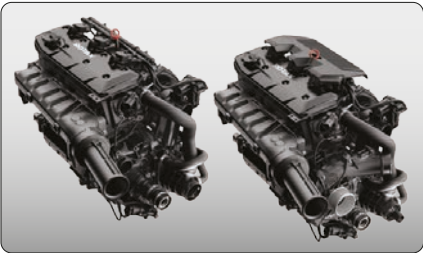
ROTAX® 1630 ACE™ - 230 The 230hp engine with a supercharger and external intercooler, optimised to run on regular fuel.
